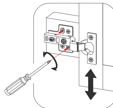
Vertical adjustment Réglage vertical Ajuste vertical
